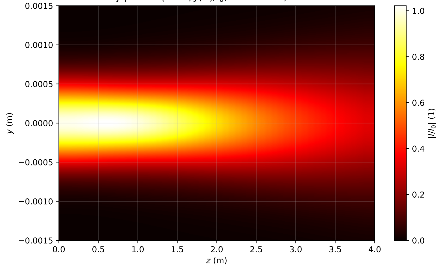
Intensity profile I(x=0, y, z)/I_0 , P_{in}=0.4P_{cr} , artificial time
